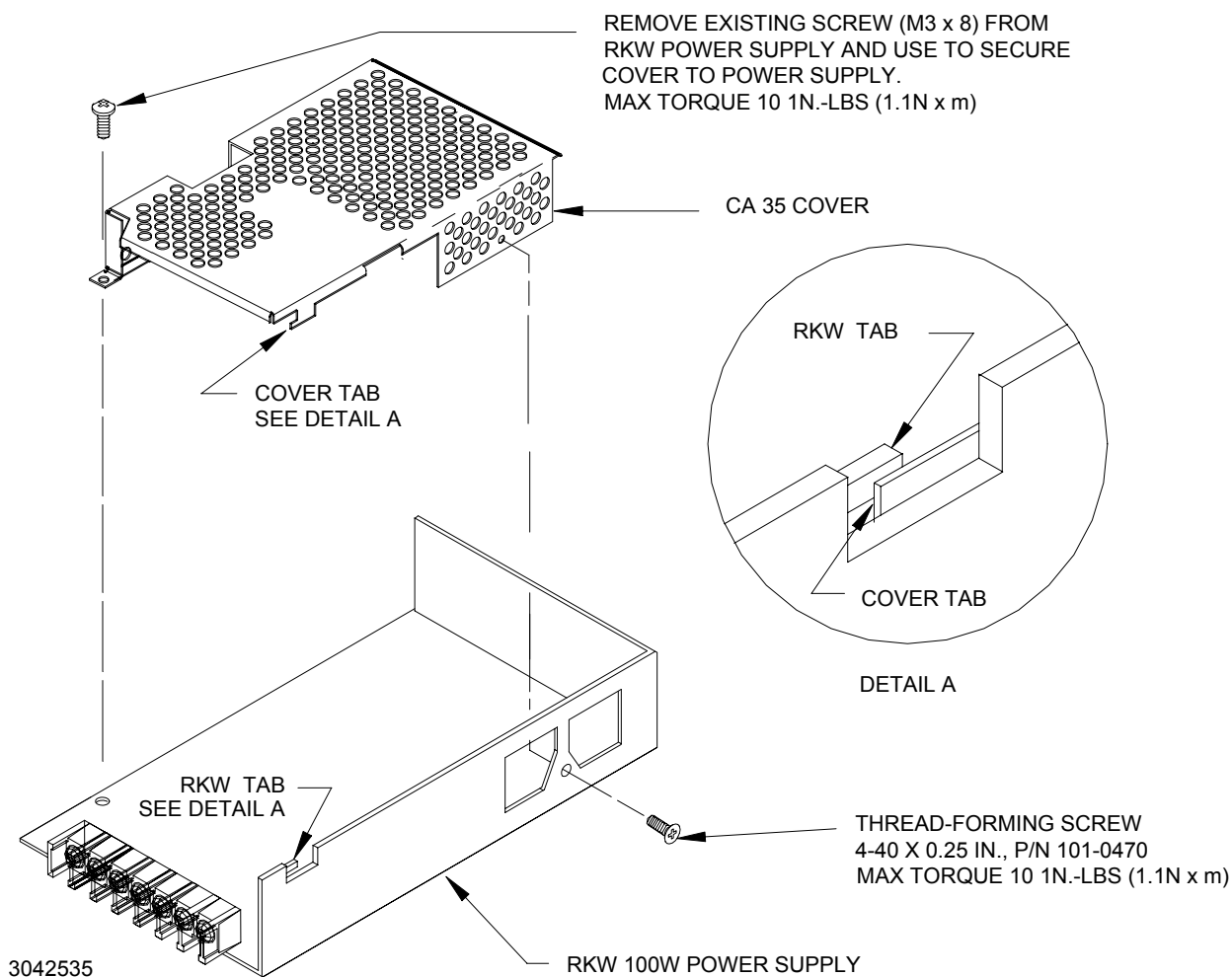
FIGURE 1. CA 35-R COVER INSTALLATION
